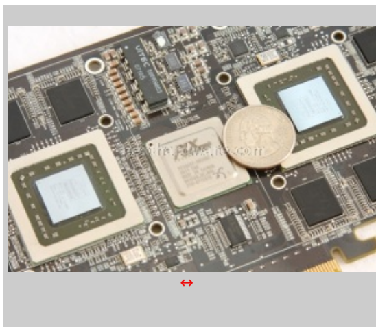
RV770 GPUs e il PLX PCIe v1.1 bridge chip
