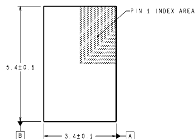
TOP SIDE OF PACKAGE
