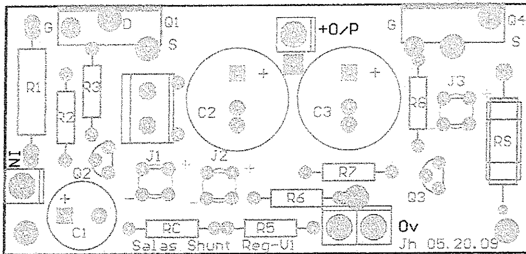
Components - Top Layer
