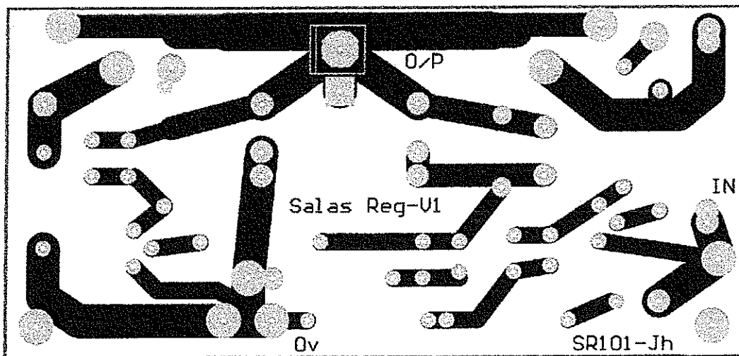
Copper Layer - Bottom View
